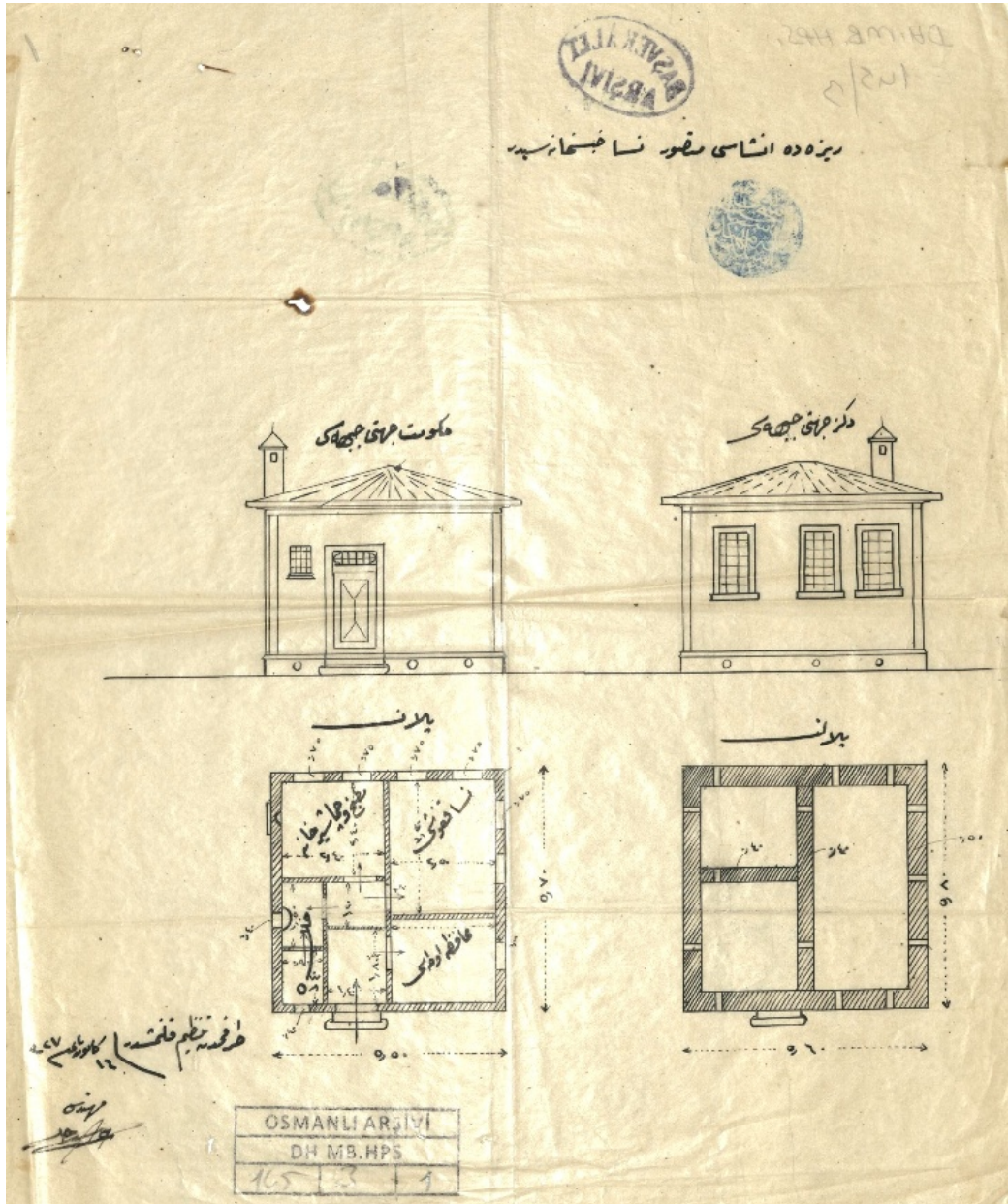
Görsel 3. Rize Nisa Hapishanesi Projesi (BOA. DH. MB. HPS. 145/3)
